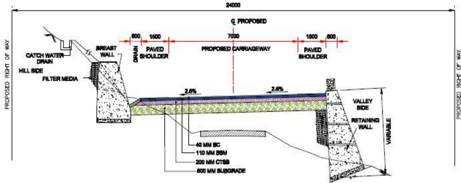
TCS 1 Two Lane With Paved Shoulder Raised Portion(Hill Section)
